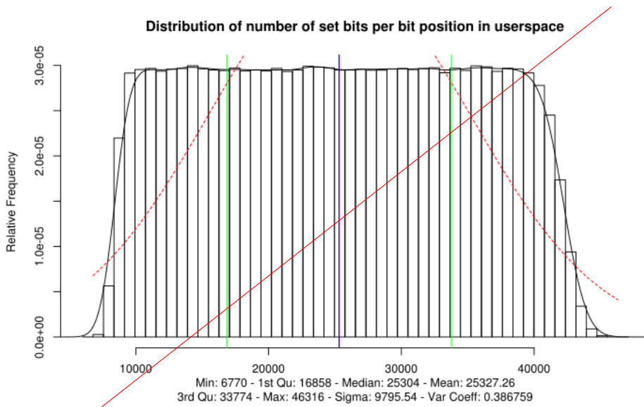
Figure 4.3: Bit sum of set bits per bit position in user space
