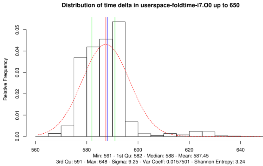
Figure 5.1: Distribution of timing variations over hash loop in user space
