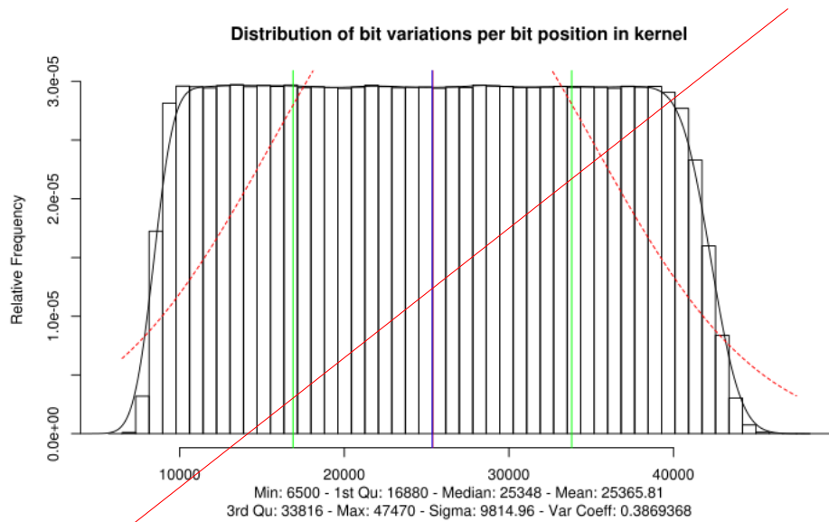
Figure 4.6: Bit sum of bit variations per bit position in kernel space
