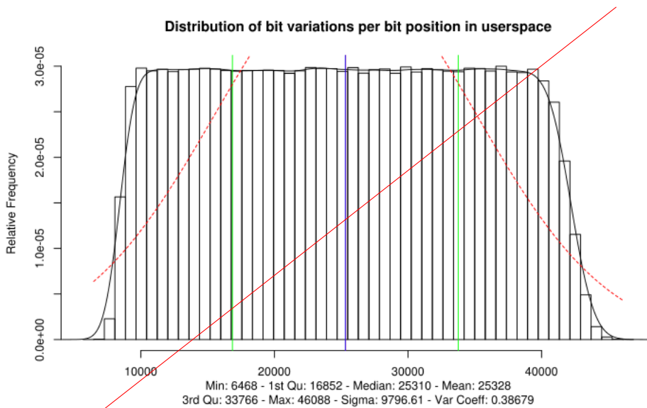
Figure 4.5: Bit sum of bit variations per bit position in user space
