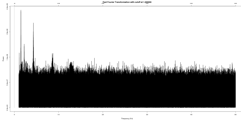
Figure 5.4: FFT of hash loop and memory access loop counts
