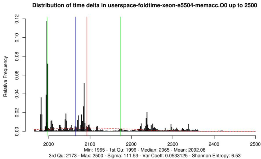
Figure 6.9: hash loop with memory accesses on Intel Xeon E5504
