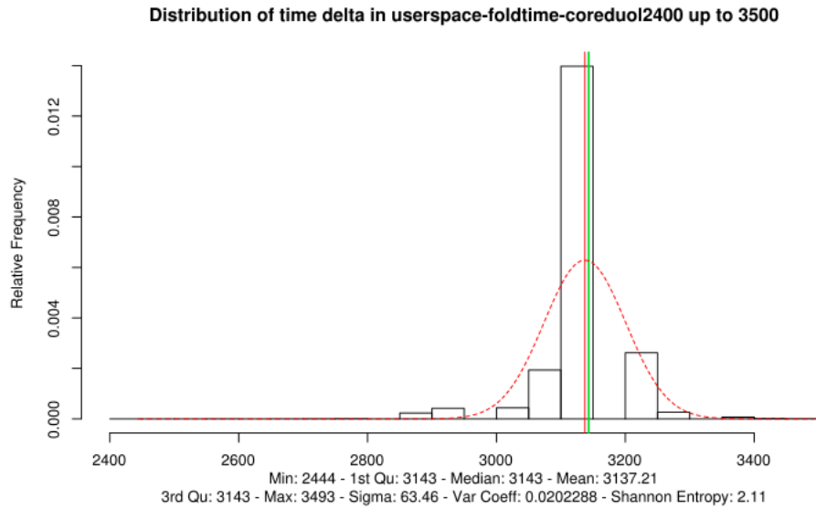
Figure C.14: Entropy over hash loop in user space on Intel Core Duo L2400
