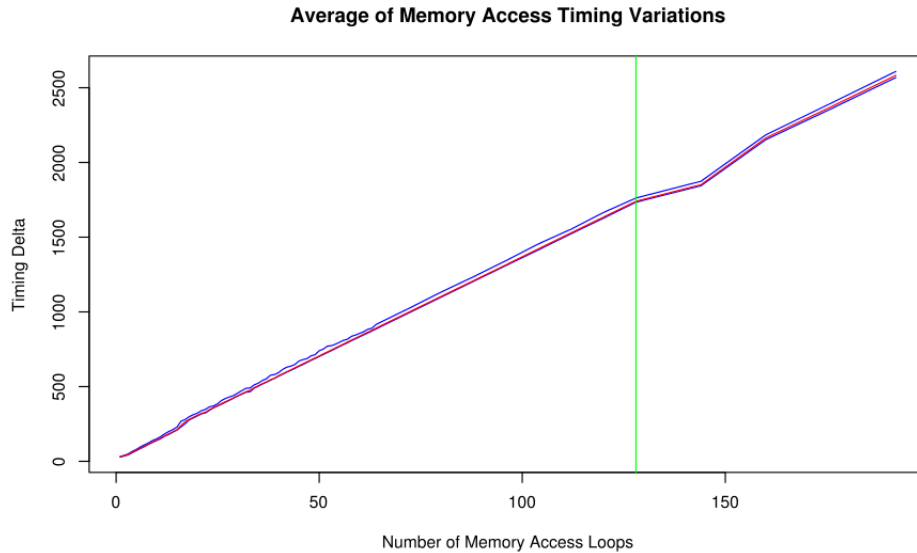
Figure 6.2: Average time duration for memory accesses
