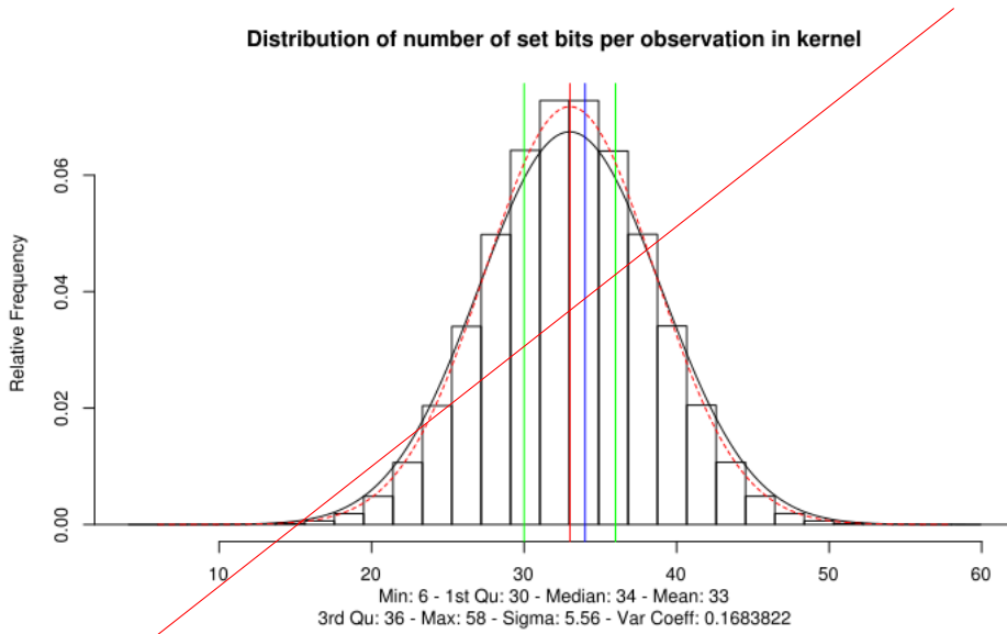
Figure 4.2: Bit sum of last round of entropy collection loop kernel space
