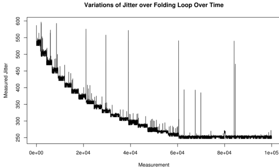
Figure 5.5: Variations of the execution time jitter over time when performing LFSR loop jitter measurements with Frequency Scaling / Power Management
