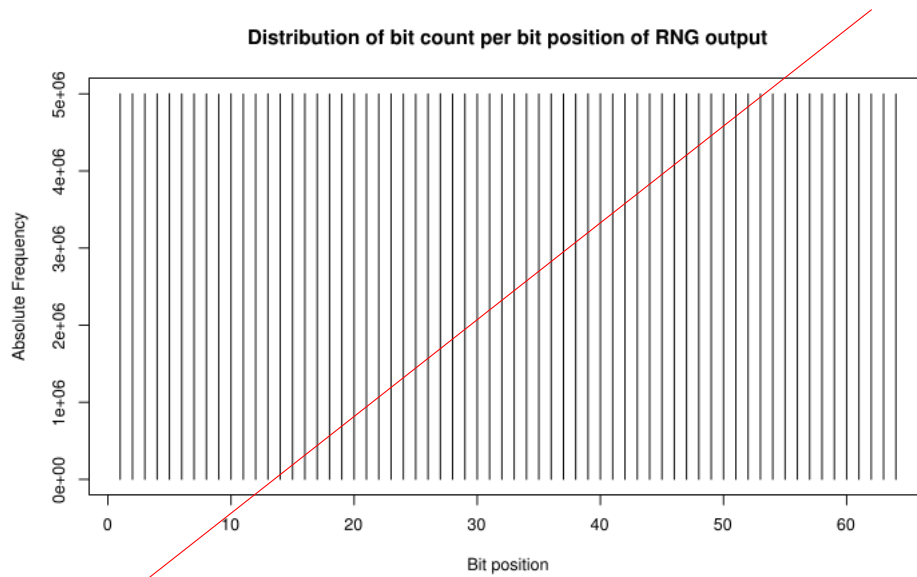
Figure 4.7: Distribution of bit count per bit position of RNG output
