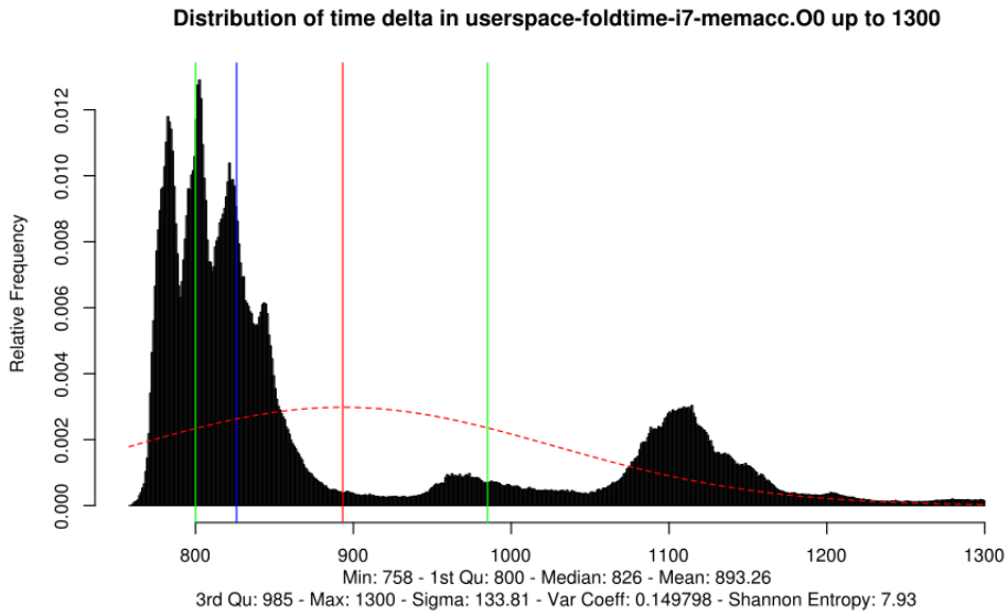
Figure 5.2: Distribution of timing variations over hash loop and constant memory access in user space
