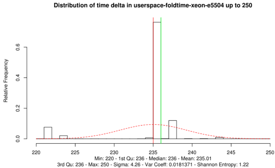
Figure 6.8: hash loop without memory accesses on Intel Xeon E5504 – lower boundary
