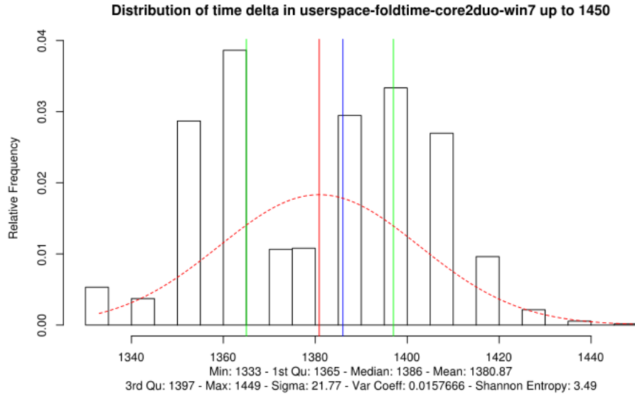
Figure C.13: Entropy over hash loop in user space on Intel Core 2 Duo with Windows – without optimizations
