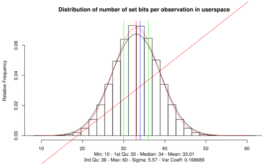
Figure 4.1: Bit sum of last round of entropy collection loop user space
